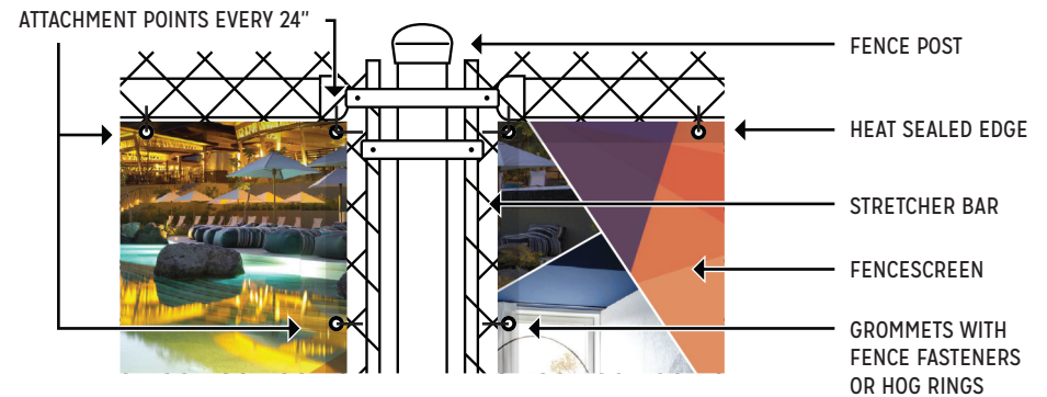
Attachment Enlargement
