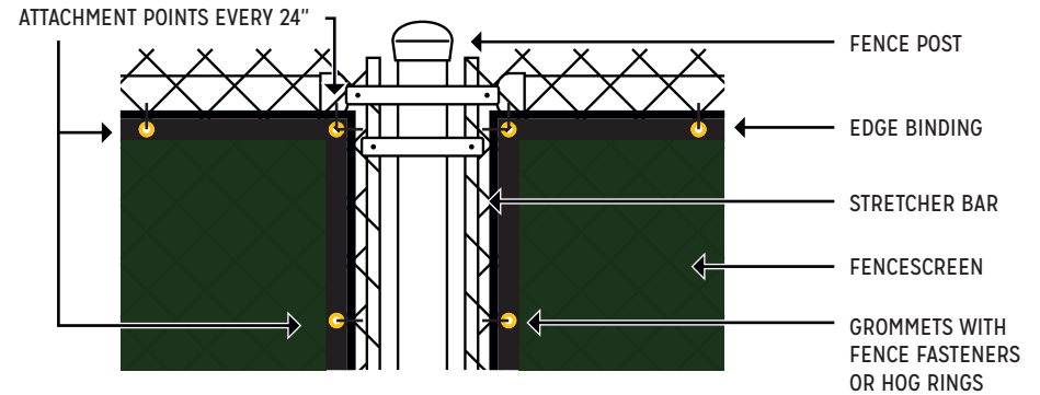
Attachment Enlargement
