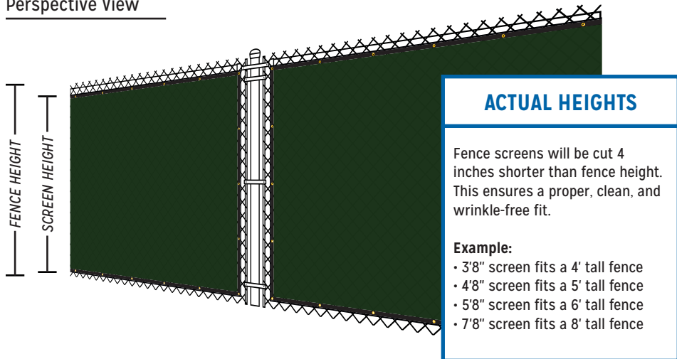
Perspective View
