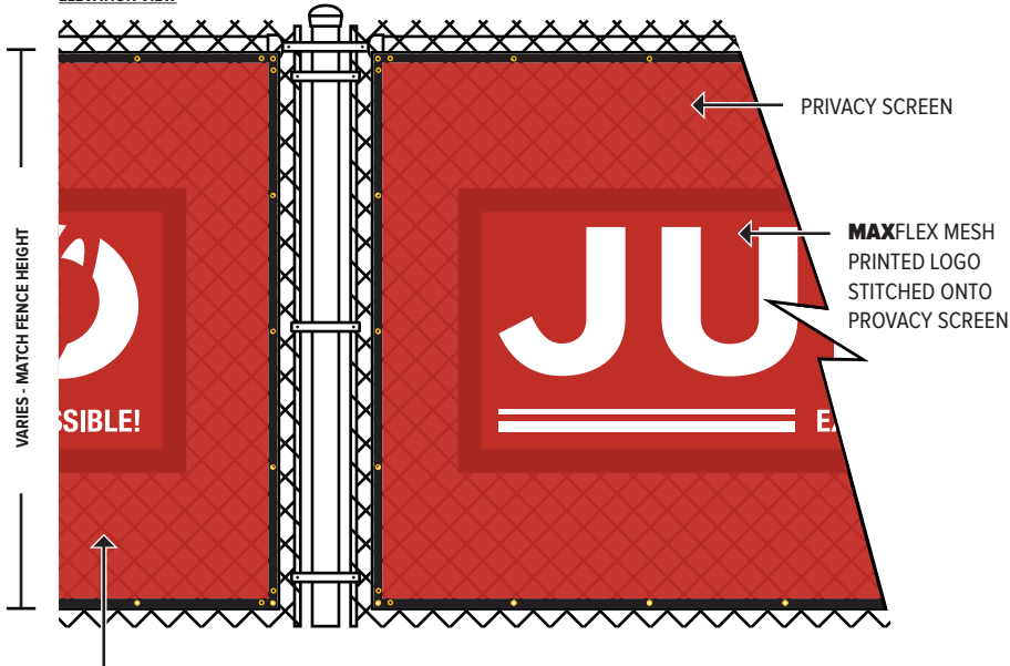
ELEVATION VIEW
