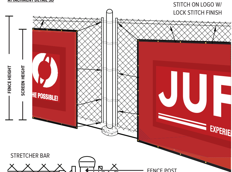
ATTACHMENT DETAIL 3D
