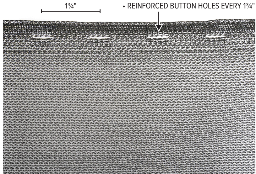
MATERIAL DETAIL
