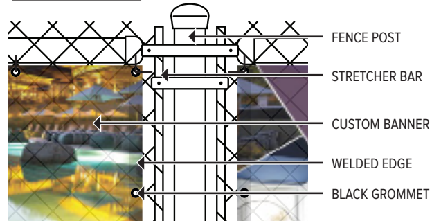
ATTACHMENT ENLARGEMENT
