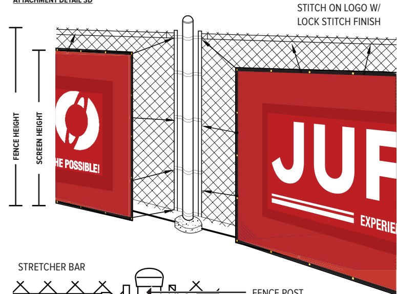
ATTACHMENT DETAIL 3D
