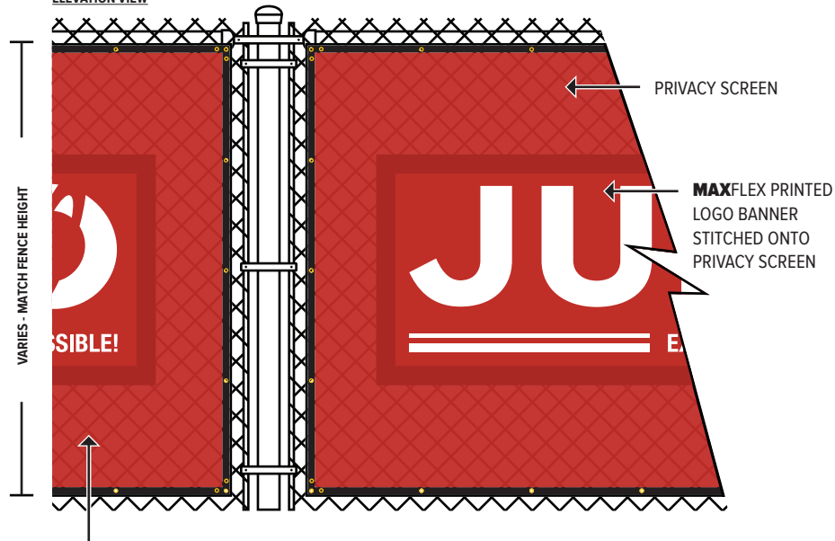
ELEVATION VIEW
