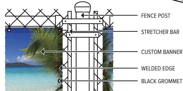
ATTACHMENT ENLARGEMENT
