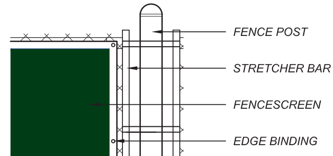
ATTACHMENT ENLARGEMENT
