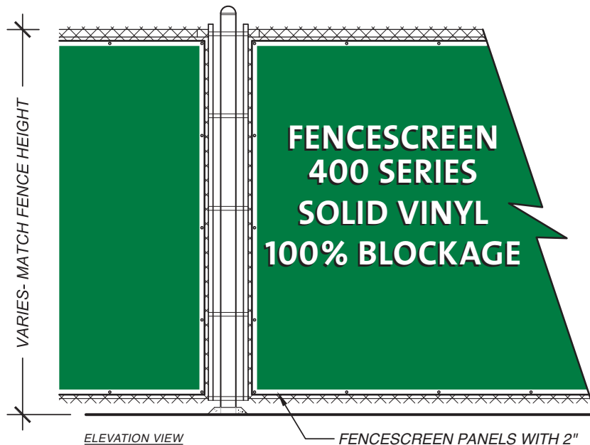
ELEVATION VIEW
